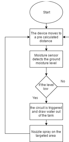
Fig. 3 Flowchart of the proposed system
