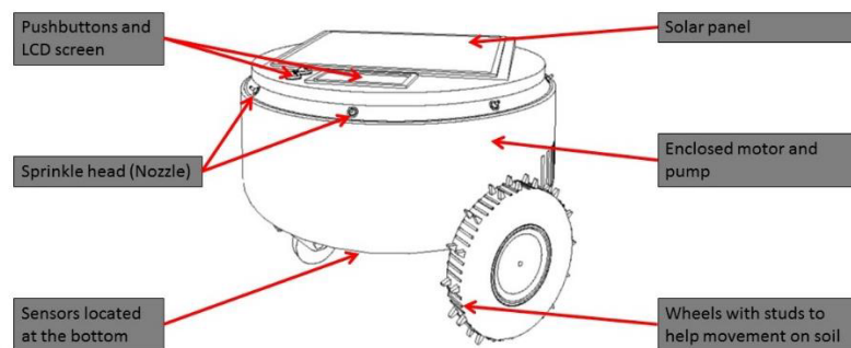
Fig.8 Illustration of the product design
