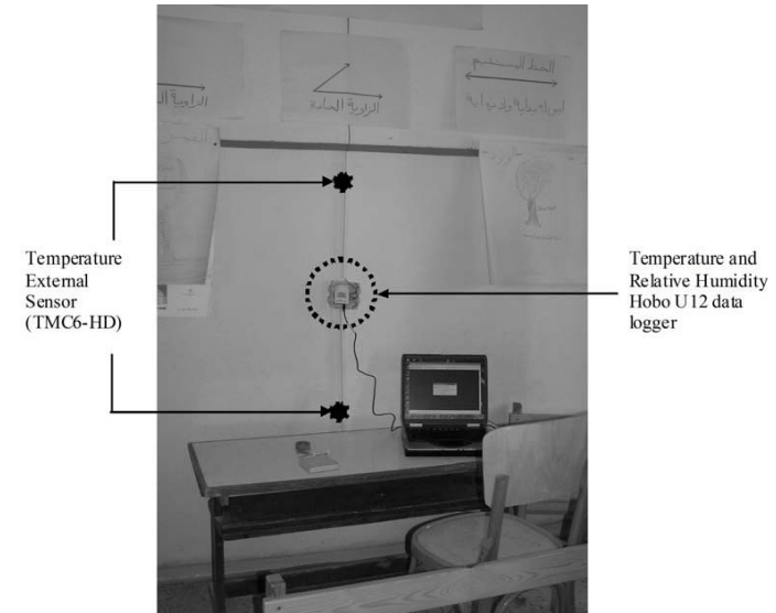
Figure 5: Hobo U12 and sensors on the back wall of the classroom
