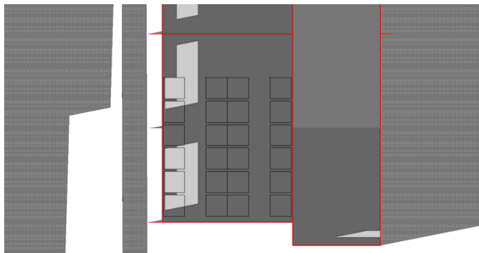
Figure 6: Solar penetration at 14:00 during mid May
