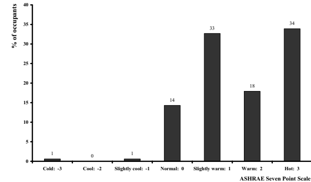
Figure 6: Percentage of occupants' response at each point on ASHRAE Seven Point Scale
